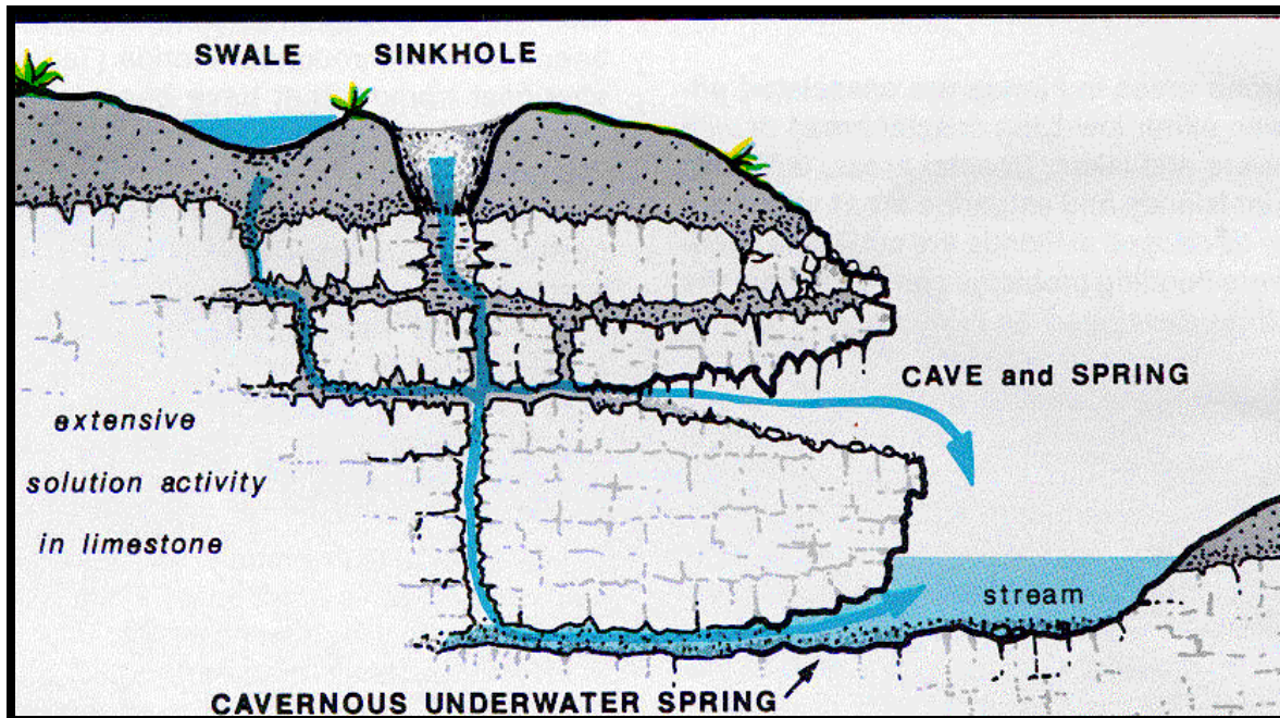
Figure 2. Advance Karst Development (Lane,1994).
